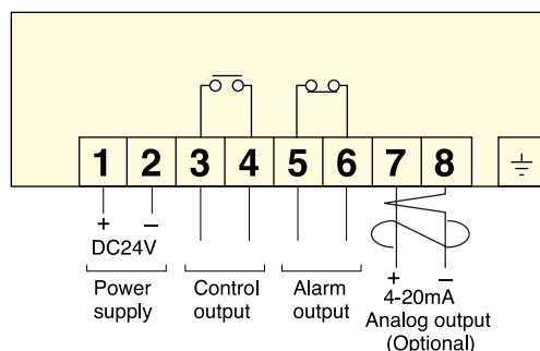
Selection of detection mode and relay configuration
