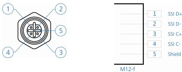
Figure 9 : Connection diagram LDM301S SSI
